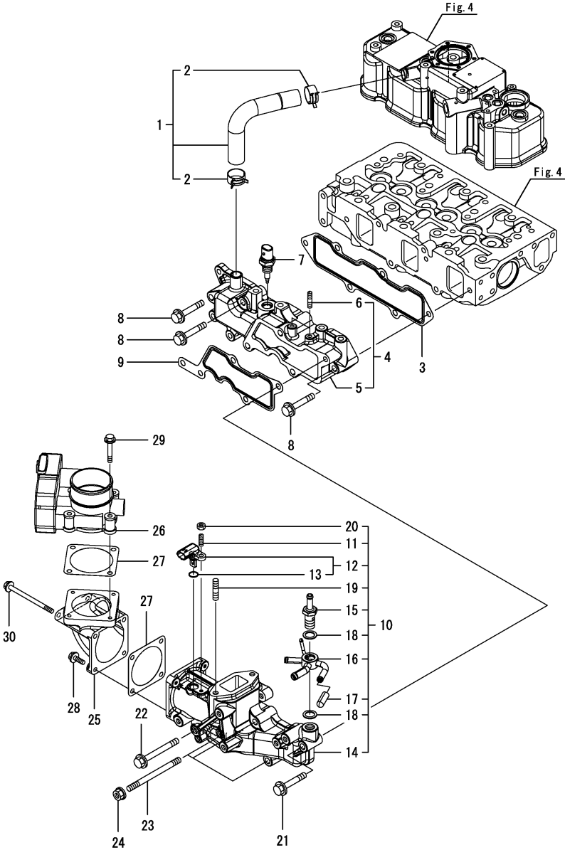
Fig.5. SUCTION MANIFOLD
