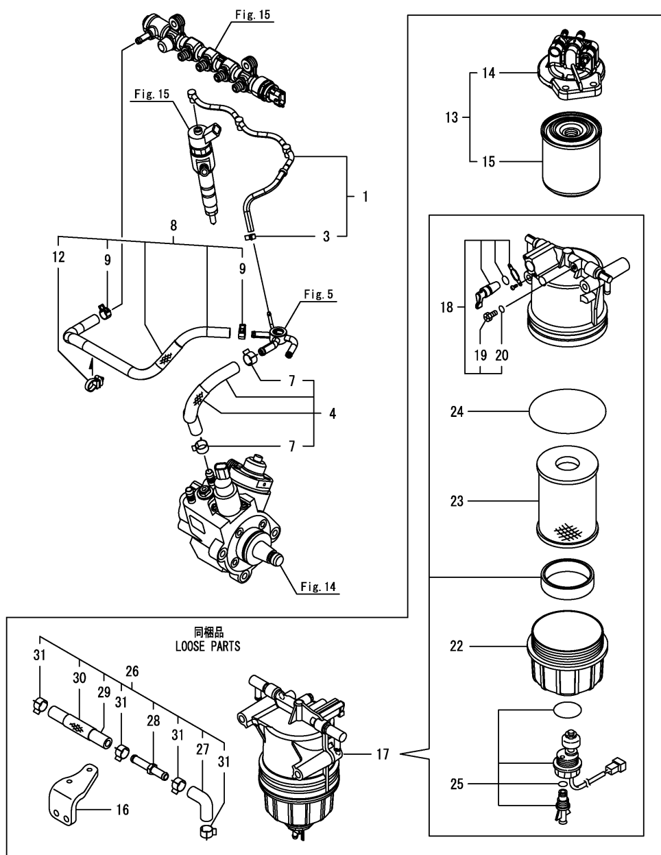
Fig.16. FUEL PIPE
