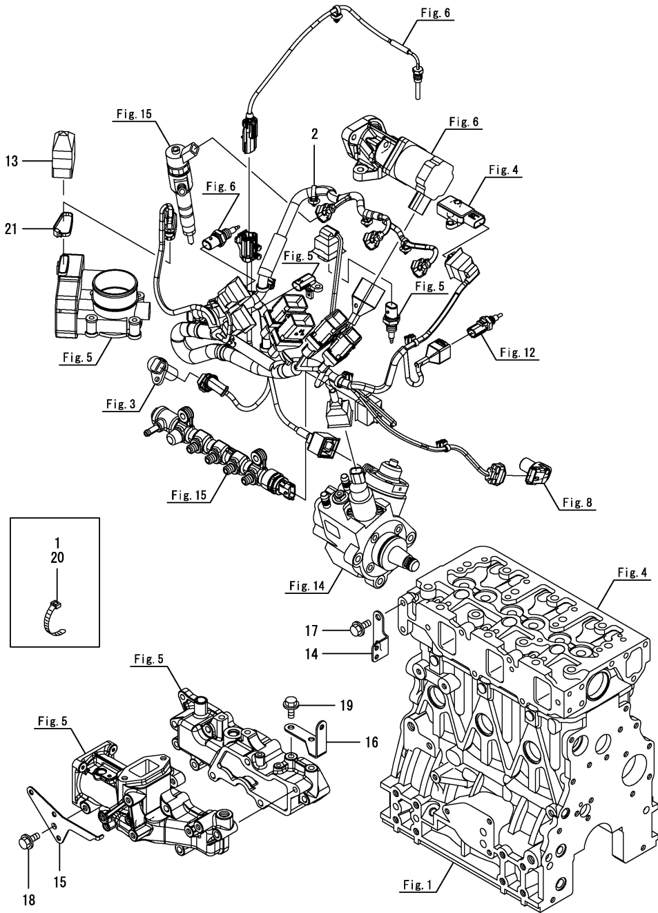
Fig.21. ELECTRIC PARTS
