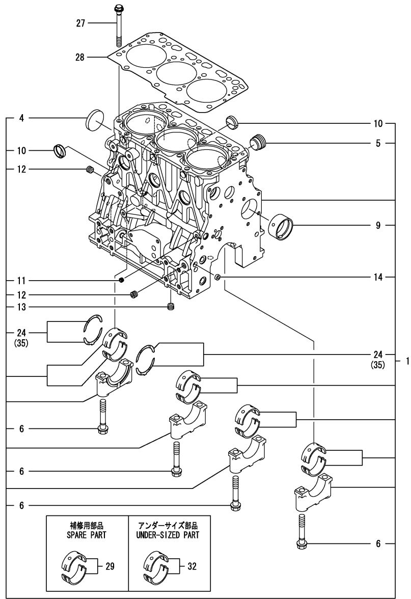
Fig.1. CYLINDER BLOCK
