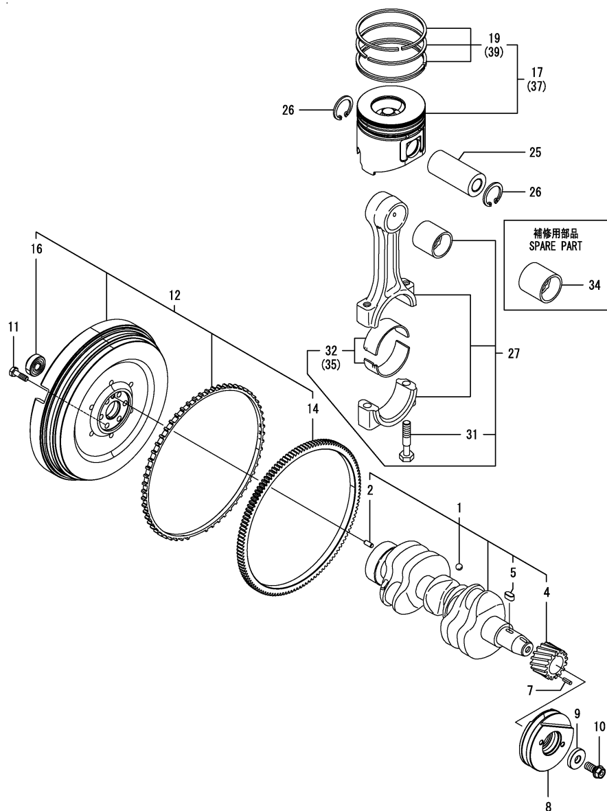
Fig.9. CRANKSHAFT & PISTON
