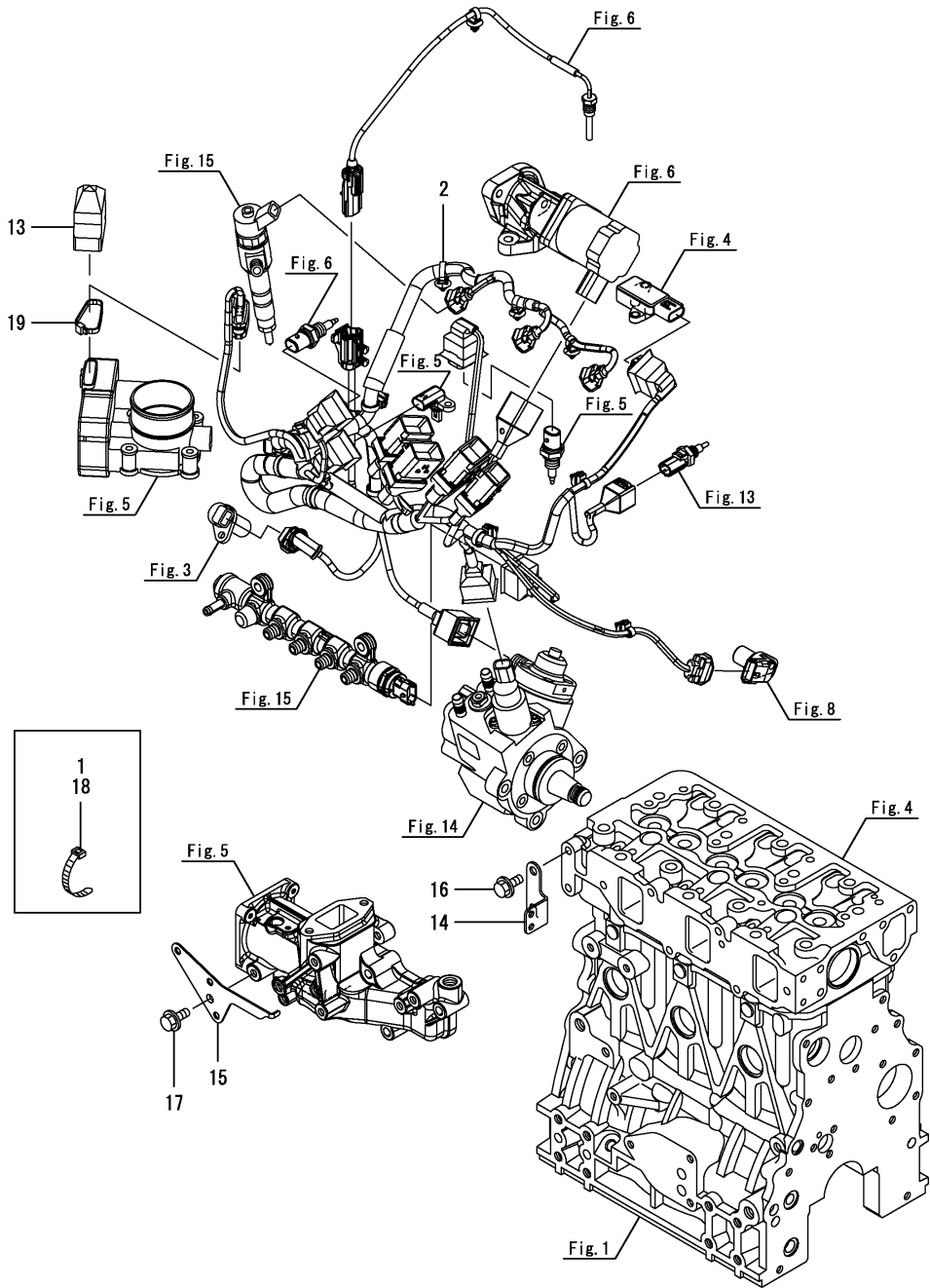
Fig.22. ELECTRIC PARTS
