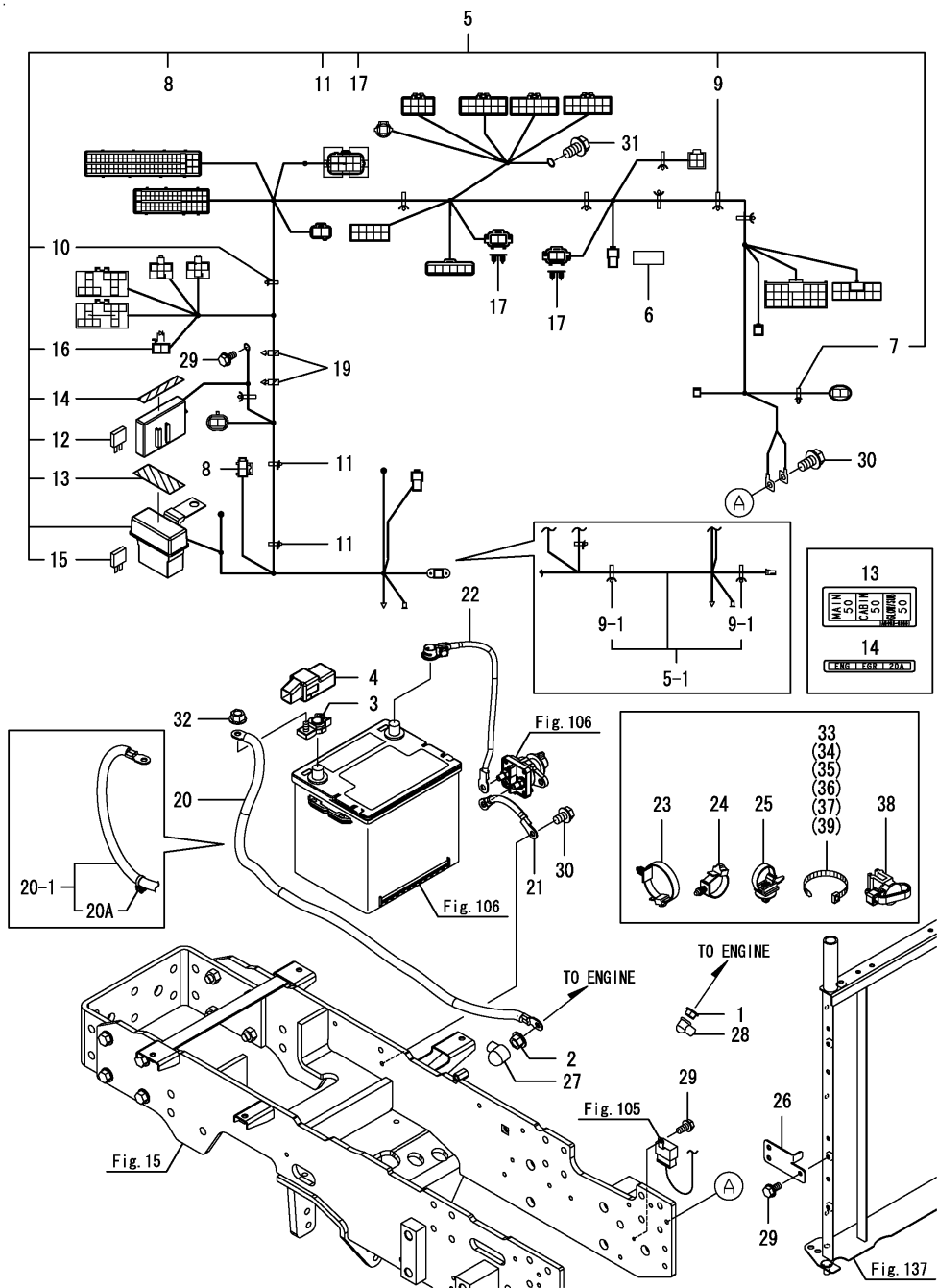
Fig.102. WIRE HARNESS(ENGINE)(CABIN)
