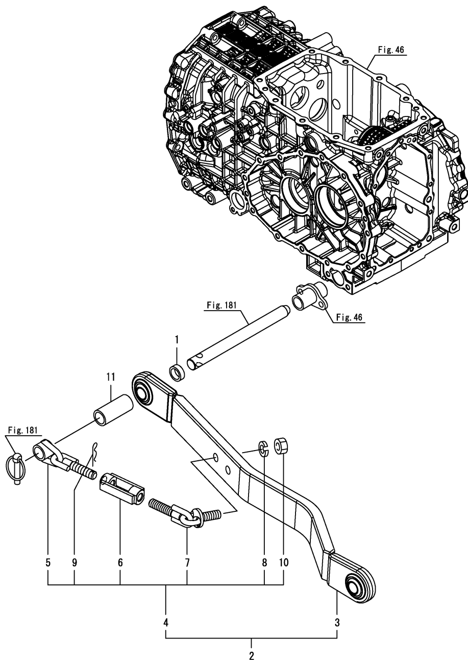
Fig.180. LOWER LINK
