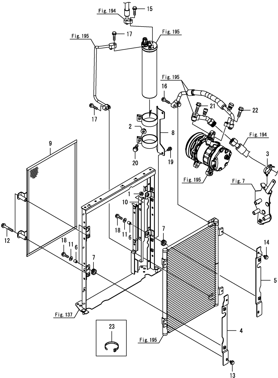
Fig.3. COOLER(ACCESSORIES)(CABIN)
