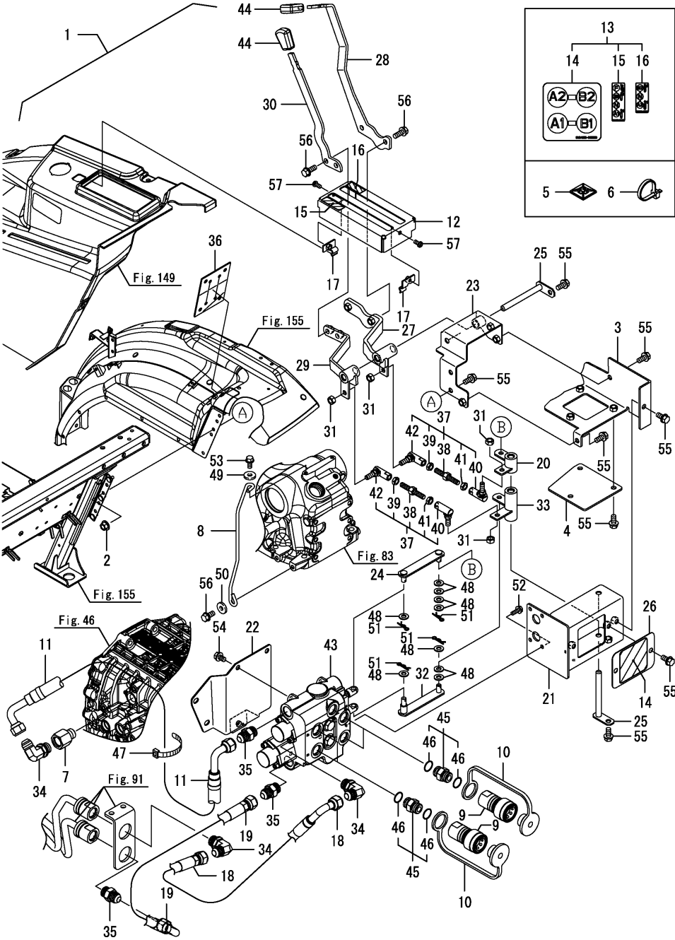
Fig.229. CONTROL KIT
