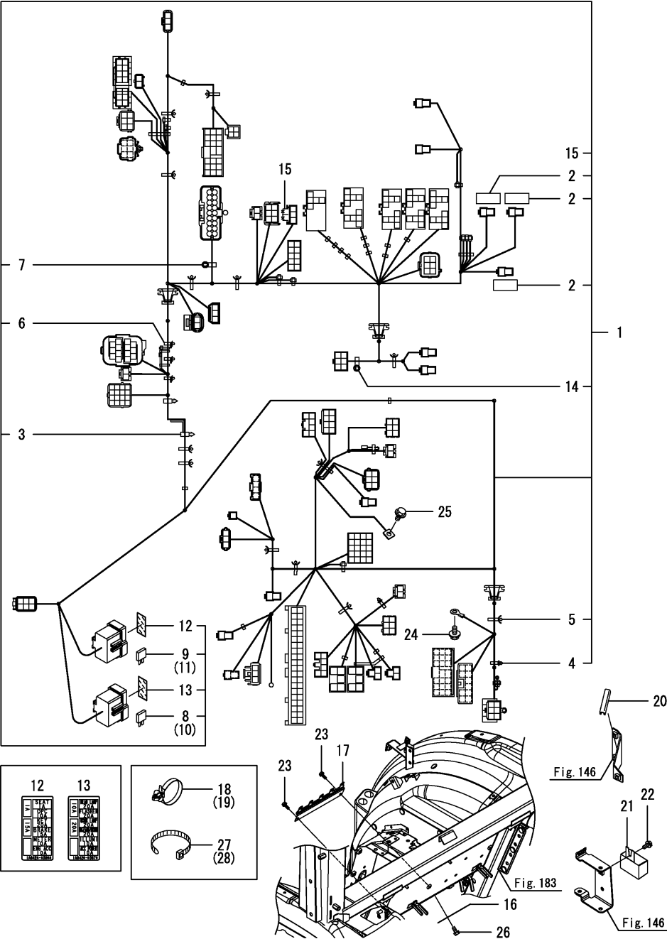
0CNP6-M06360 ELECTRICAL PARTS Fig.105. WIRE HARNESS(FLOOR)(CABIN)
