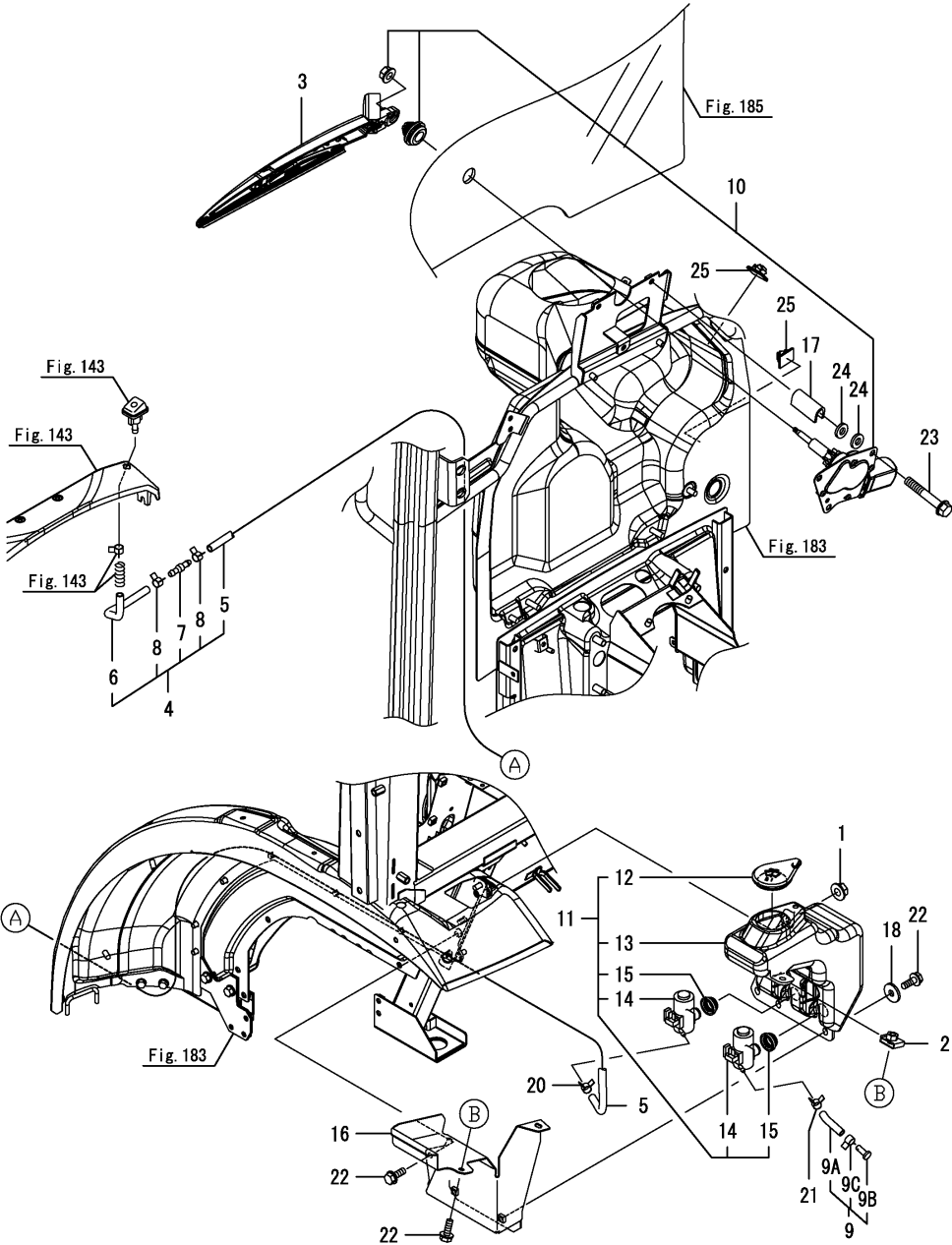
Fig.192. FRONT WIPER
