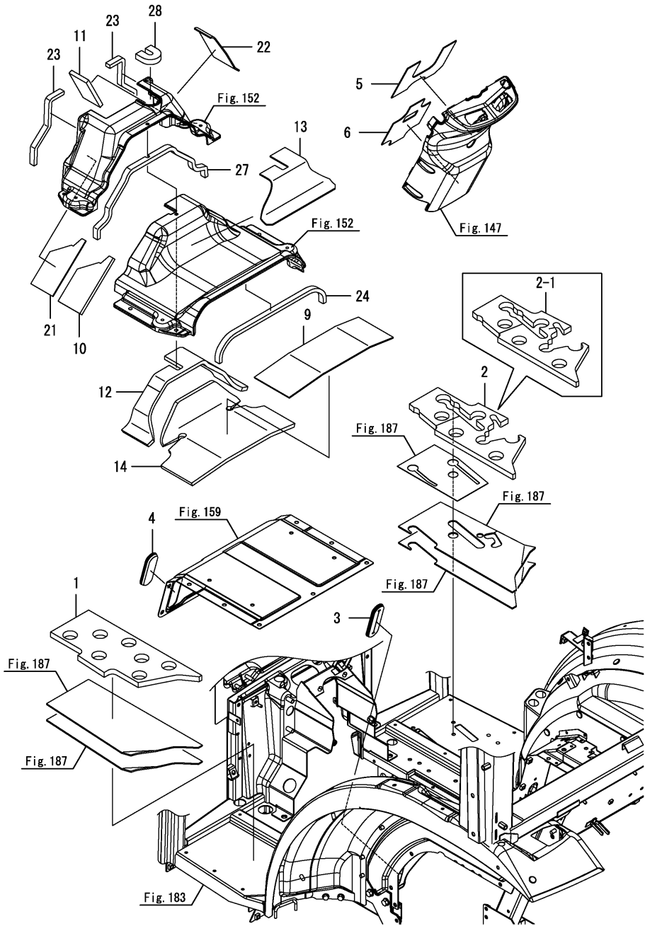
Fig.188. CABIN SEAL(2)
