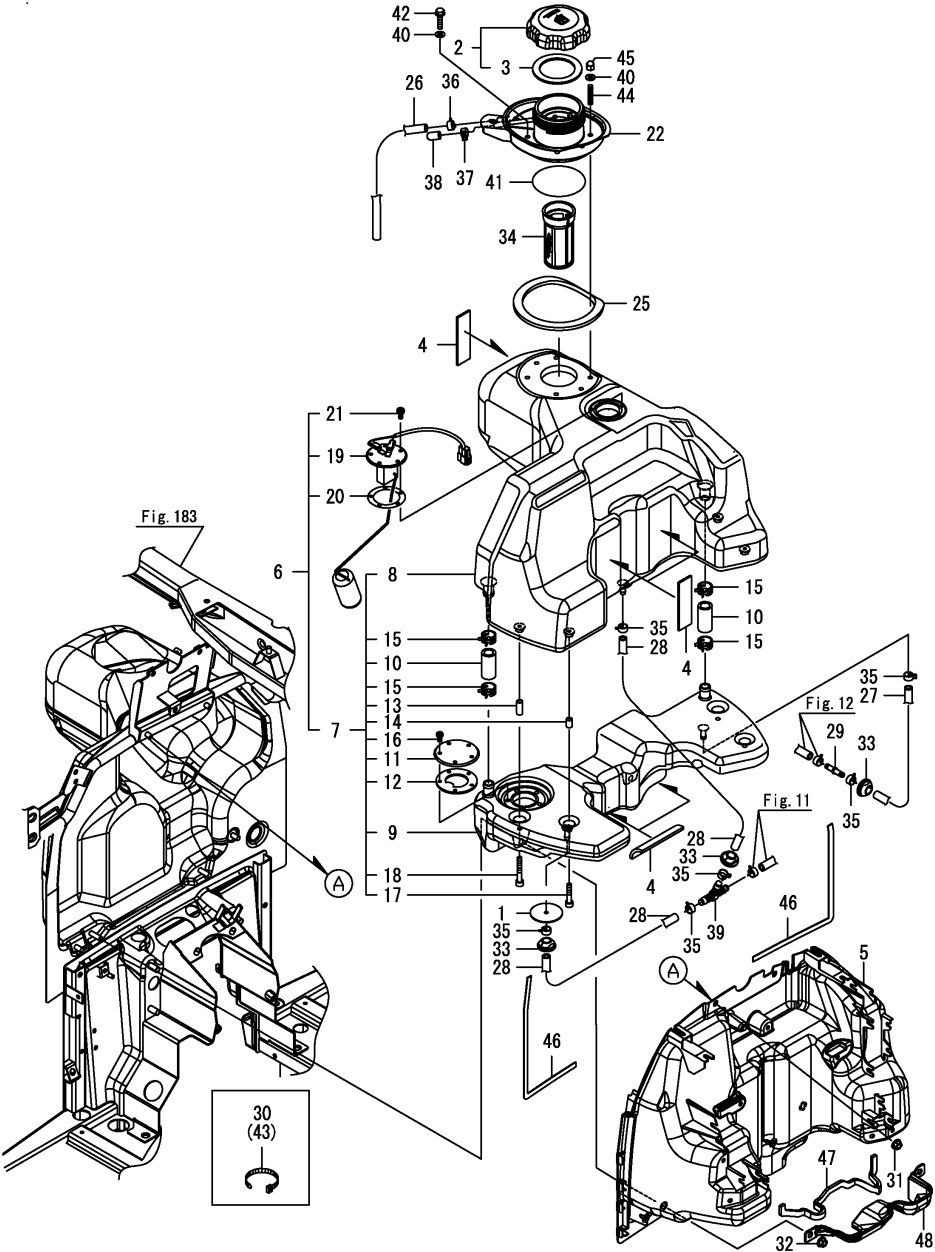
Fig.9. FUEL TANK(CABIN)
