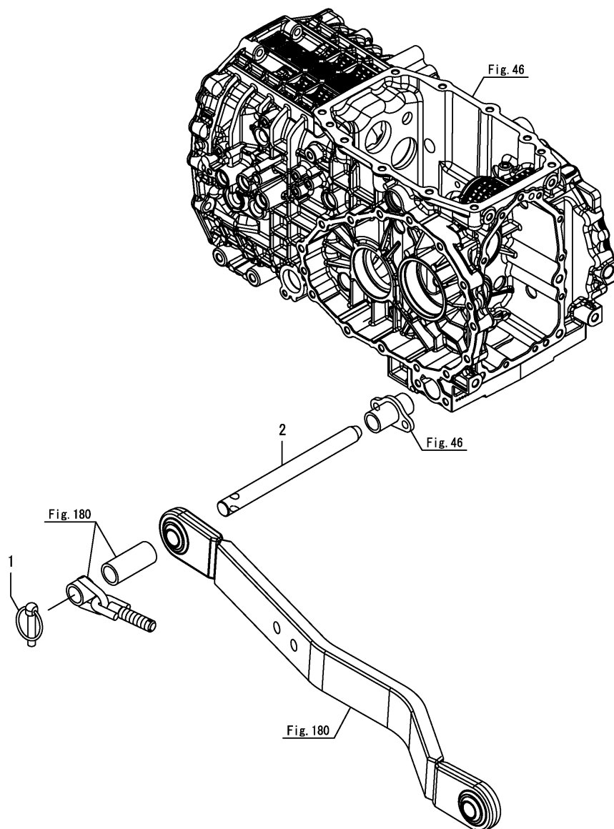
Fig.181. LOWER LINK PIN
