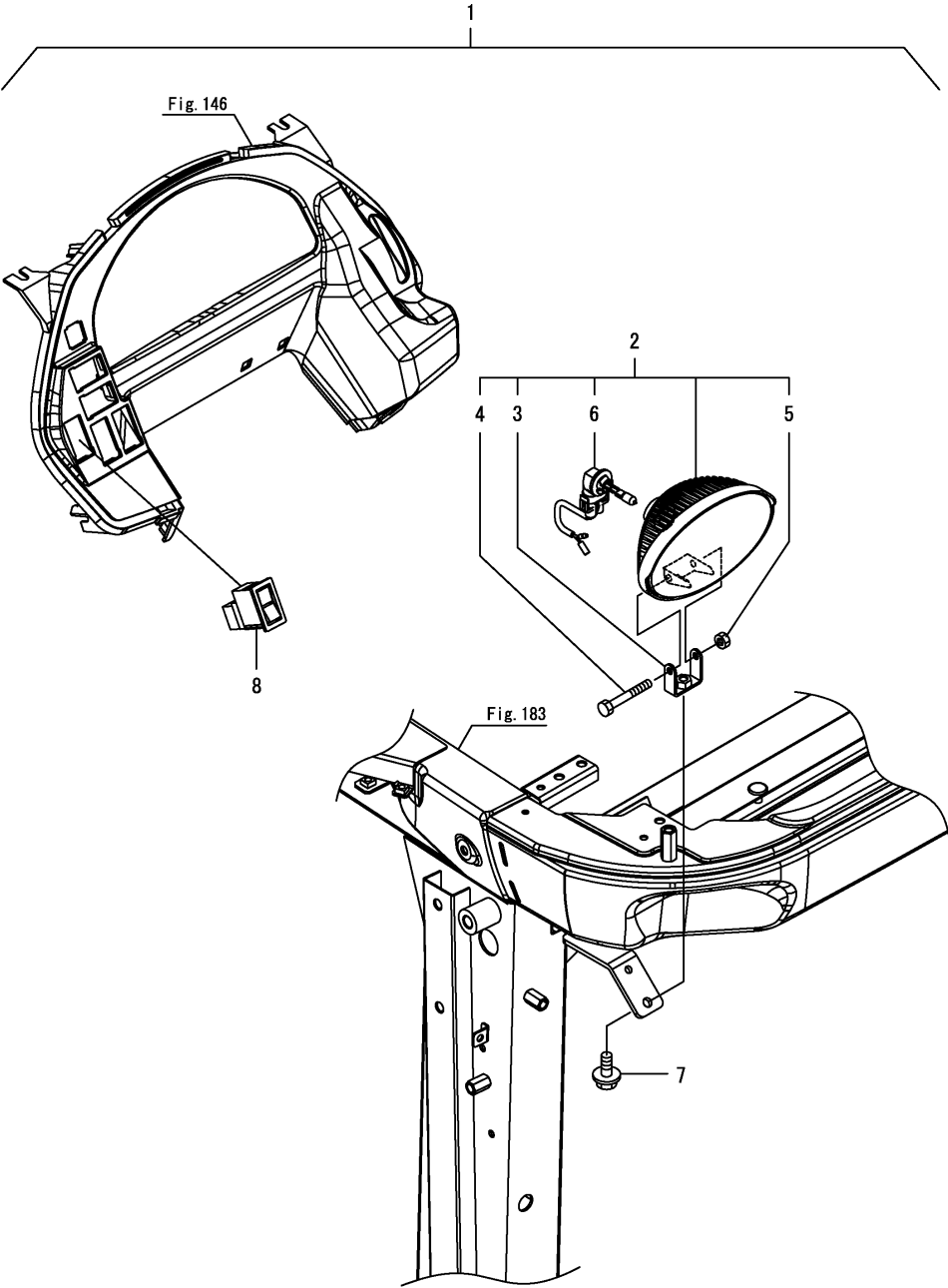
Fig.205. WORK LAMP(REAR)(CABIN)
