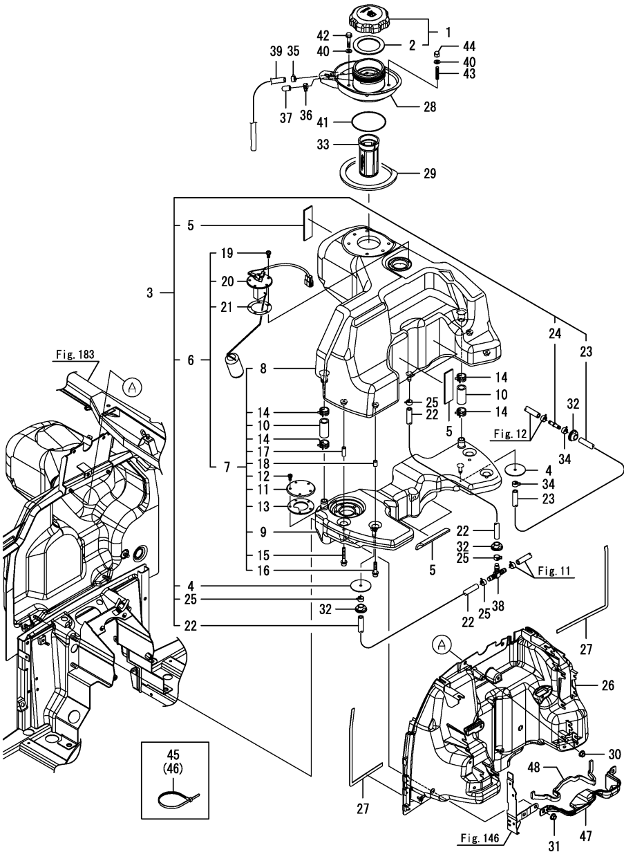
Fig.232. (9A)FUEL TANK(CABIN)
