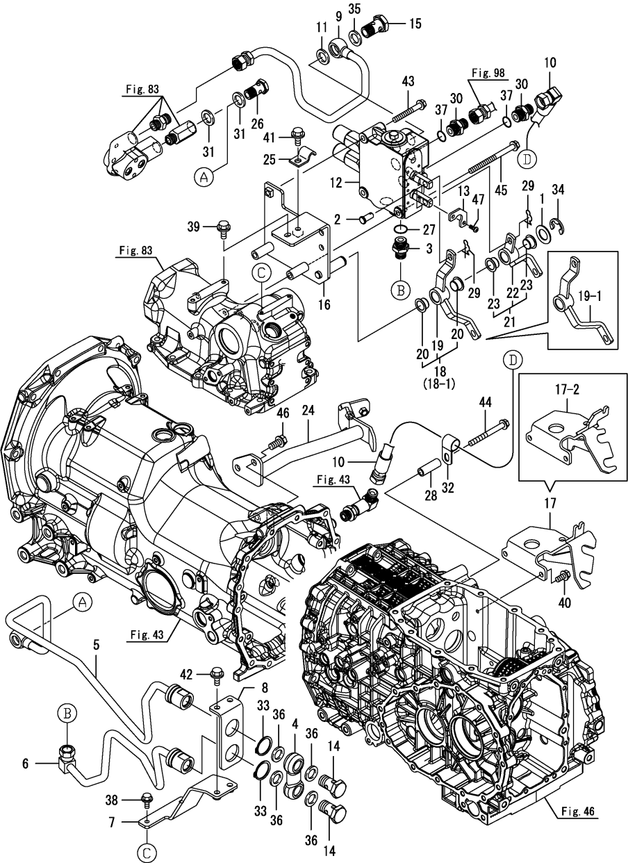
Fig.91. LOADER VALVE
