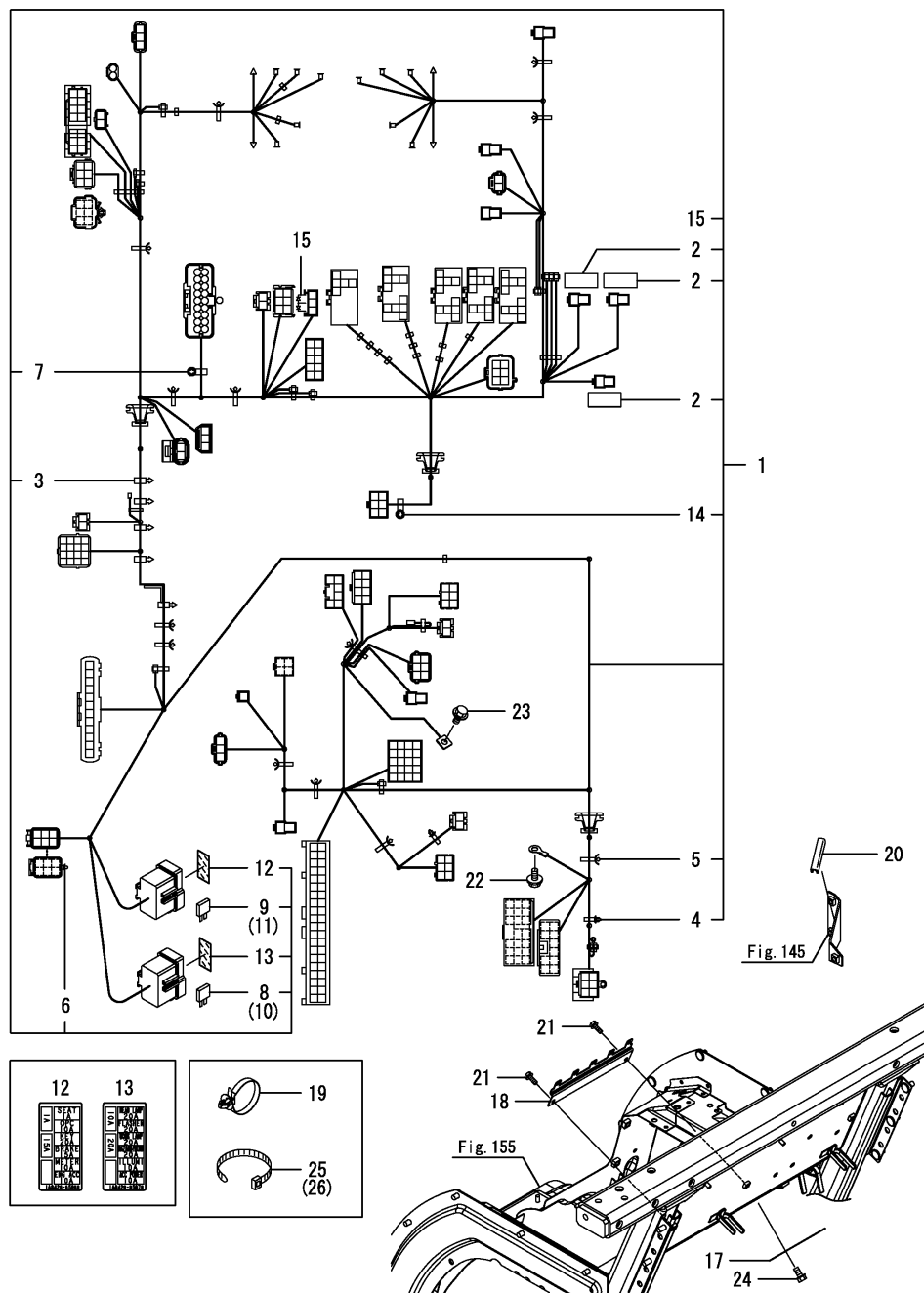
Fig.104. WIRE HARNESS(FLOOR)
