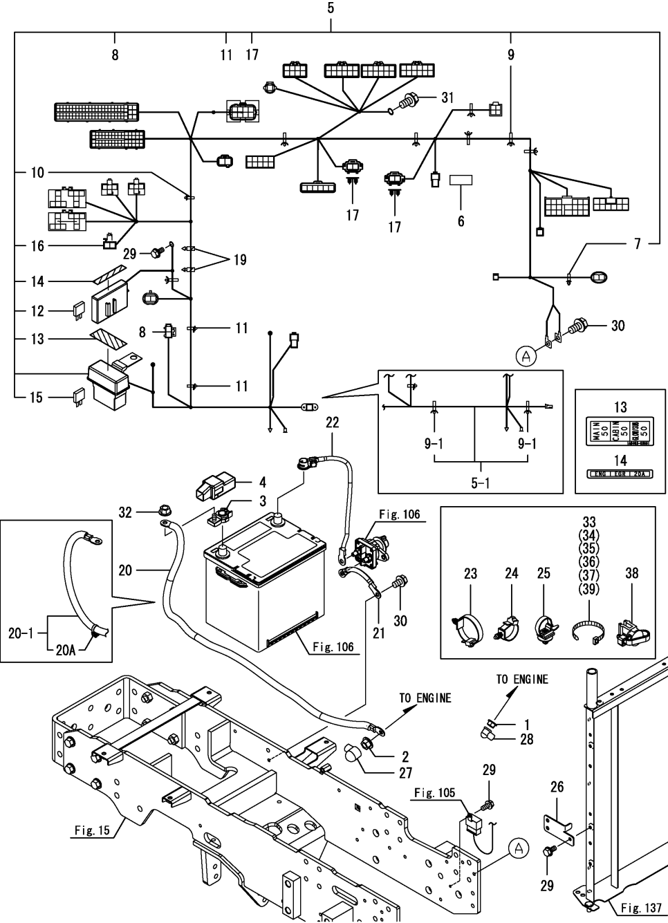
Fig.102. WIRE HARNESS(ENGINE)(CABIN)
