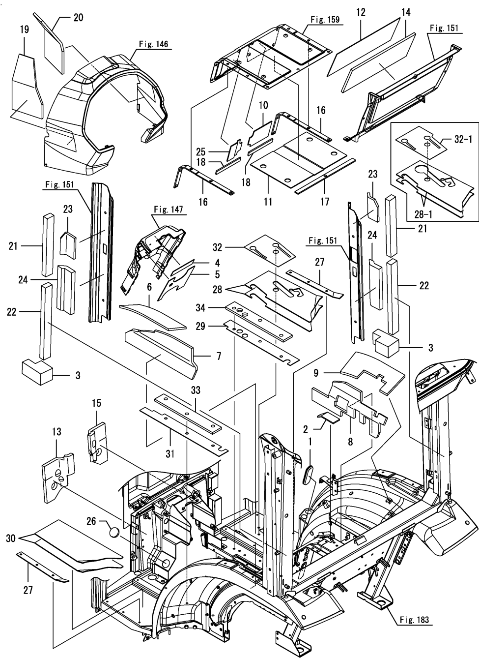
Fig.187. CABIN SEAL(1)
