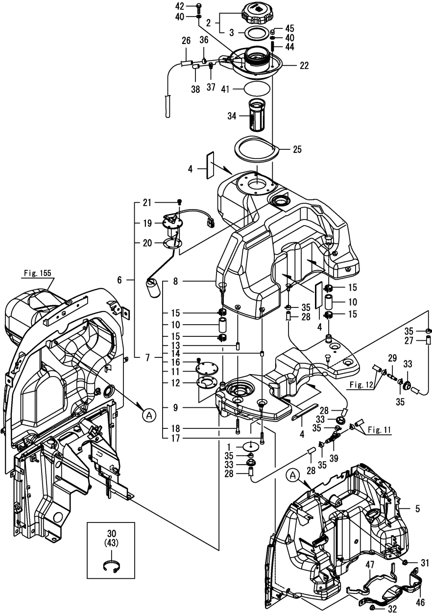
Fig.8. FUEL TANK
